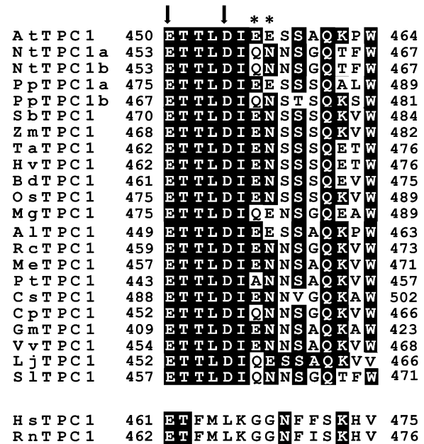
Figure 1. Alignment of the Loop between Transmembrane Domains S7 and S8 of the TPC1 Channel from Different Plant and Animal Species.
